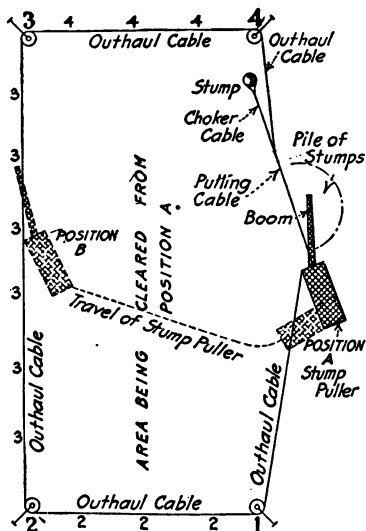
Fig. 56. Diagram Showing Field Arrangement of Clyde Land-Clearing Machine
